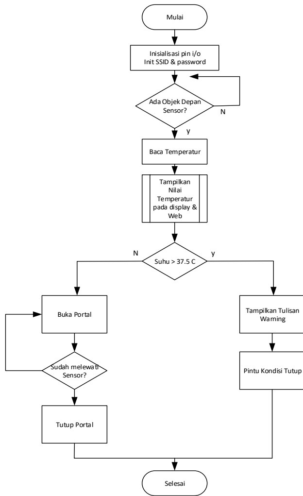
Gambar 3. Diagram Alir program
