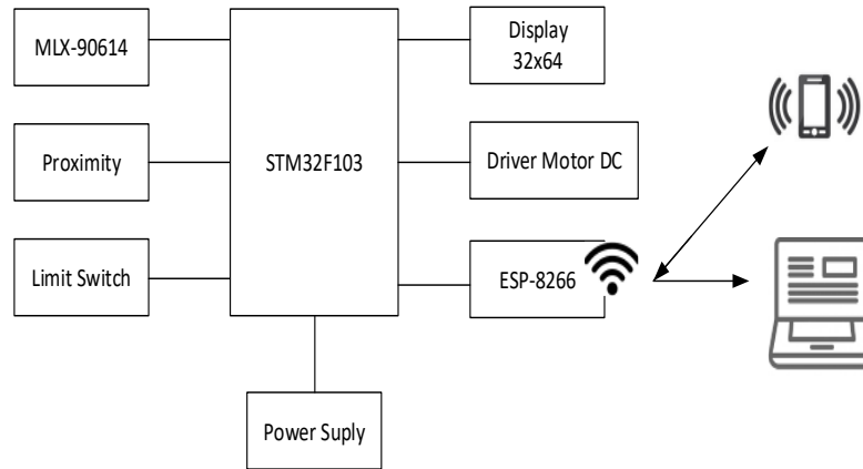
Gambar 2. Diagram blok rancangan hardware
